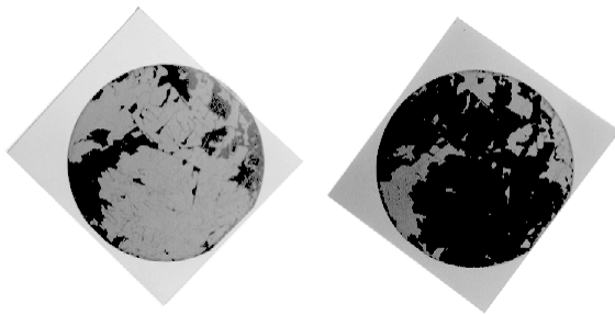
Figure 6. Intrinsic (spontaneous) Faraday rotation in an approximately 10 \mu\text{m} thick yttrium–iron garnet (YIG), diameter 70 mm, epitaxially grown on a single-crystal wafer made from yttrium–aluminium garnet (YAG). Analysers are at approximately + and -40^\circ with respect to the polarizer. The ferromagnetic domains are easily switched with a magnetic field.
