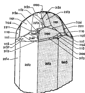
Figure 36. Incommensurate crystal \text{Au}_{1-x}\text{Ag}_x\text{Te}_2 (typical twin; Janner and Dam 1989, courtesy of OPA (Overseas Publishers Association) NV). The crystal faces are labelled with four integral indices. H_{hklm} = ha_1^* + ha_2^* + ha_3^* + m\mathbf{q} , where a_i^* are the reciprocal lattice vectors and \mathbf{q} = \alpha a_1^* + \beta a_2^* + \gamma a_3^* is a modulation vector. If at least one of the three \alpha, \beta, \gamma is irrational, the structure is incommensurably modulated.
