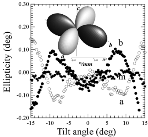
Figure 29. Tilt scans in tartaric acid samples at a wavelength of 680 nm. (a) 45° cut to approximately [100] and [010] (close to one of the optical axes), tilt axis \parallel n_\beta \approx [001] , thickness L = 0.130(5) mm; the optical rotation changes its sign close to the optical axis. (b) Cut 'on' n_\alpha = [010] (obtuse bisectrix), tilt axis \parallel n_\gamma \approx [100] , L = 0.250(5) mm. (c) Cut 'on' n_\gamma (acute bisectrix), tilt axis \parallel n_\beta \approx [001] (optic axis plane, flash figure), L = 0.360(5) . (d) Cut 'on' n_\beta , tilt axis \parallel n_\gamma , L = 0.290(5) mm. (e) 45° cut to [0\bar{1}0] and [001] , tilt axis \parallel [010](n_\alpha) , L = 0.200(5) mm; in the diagonal cut to [010] and [001] the optical rotation was found to change sign similar to the tilt scan about the optic axes. (f) The representation surface of optical rotation with respect to the physical reference system (see further Mucha et al 1997).
