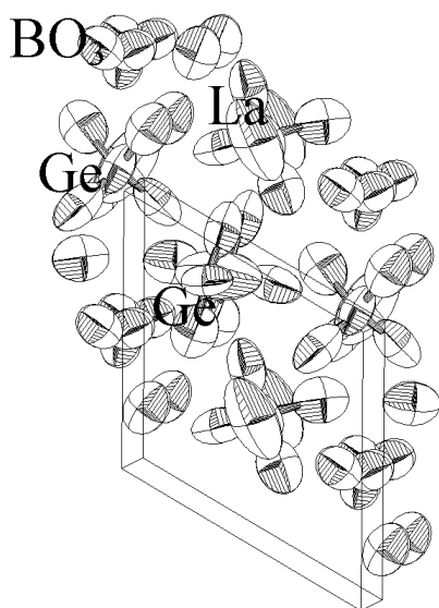
Figure 44. The structure of \text{LaBGeO}_5 ( P3_1 ) when seen towards approximately the c -axis. The dextrorotative contribution to optical rotation is dominated by the screw-axis-like sequence La–Ge–La–Ge etc. The other oxygen seem to counterbalance the dextrorotative helices.
